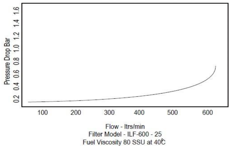
Pressure Drop Curve with Clean Element
